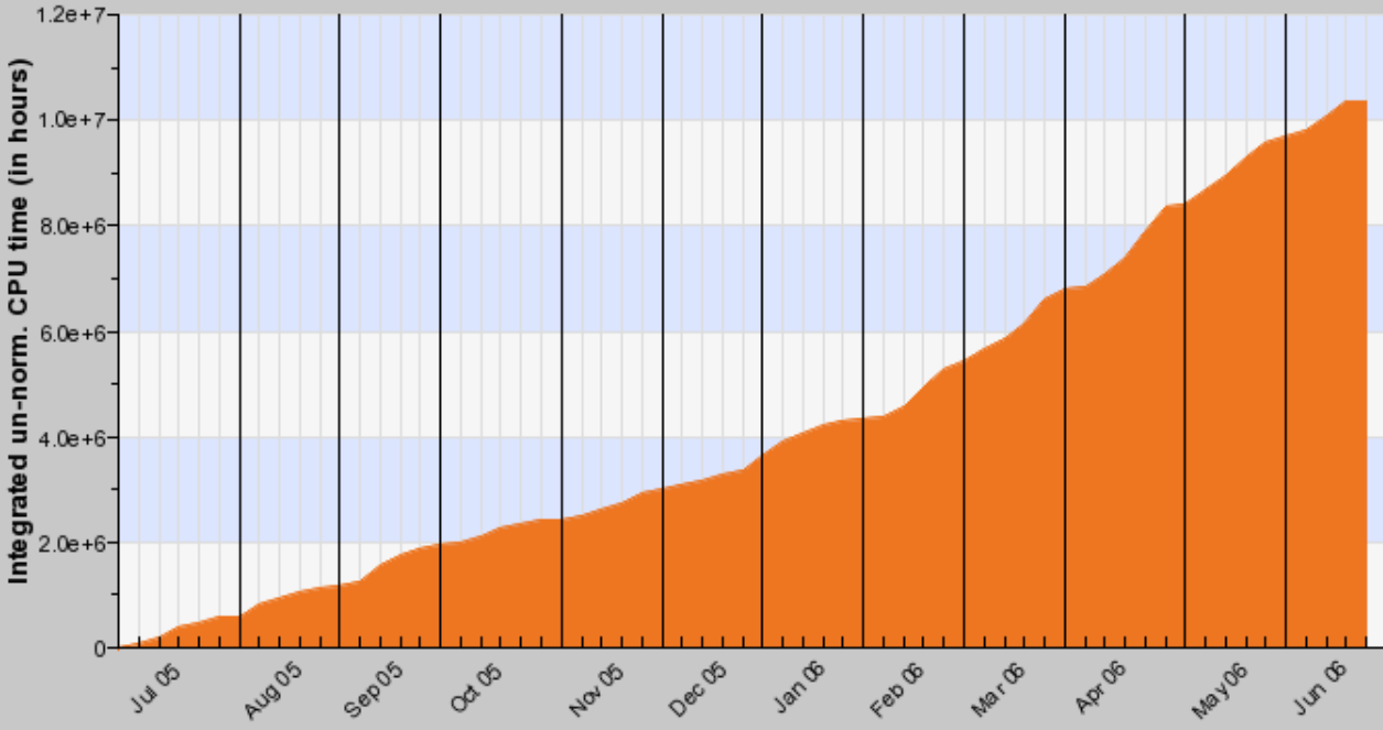
Integrated un-normalised CPU time consumed of ATLAS July 2005 - June 2006
